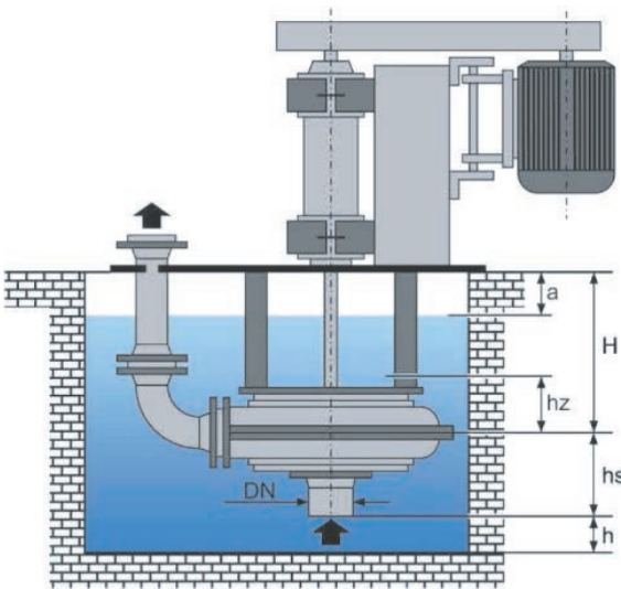
Wet installation V300 (Maximum suction height hs = 2500 mm)
