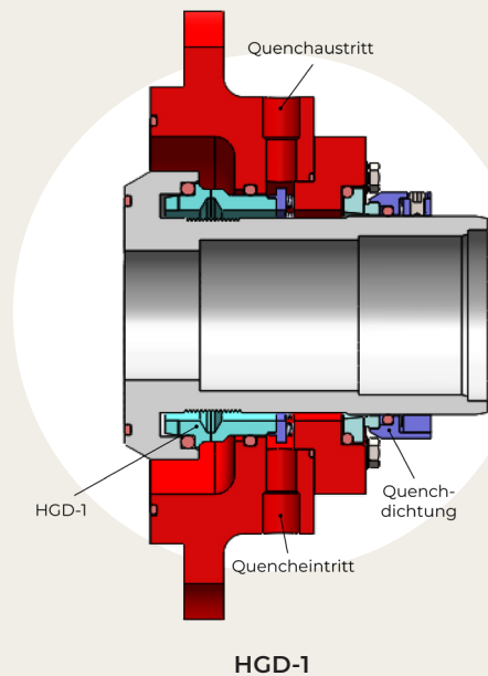
HGD-1
